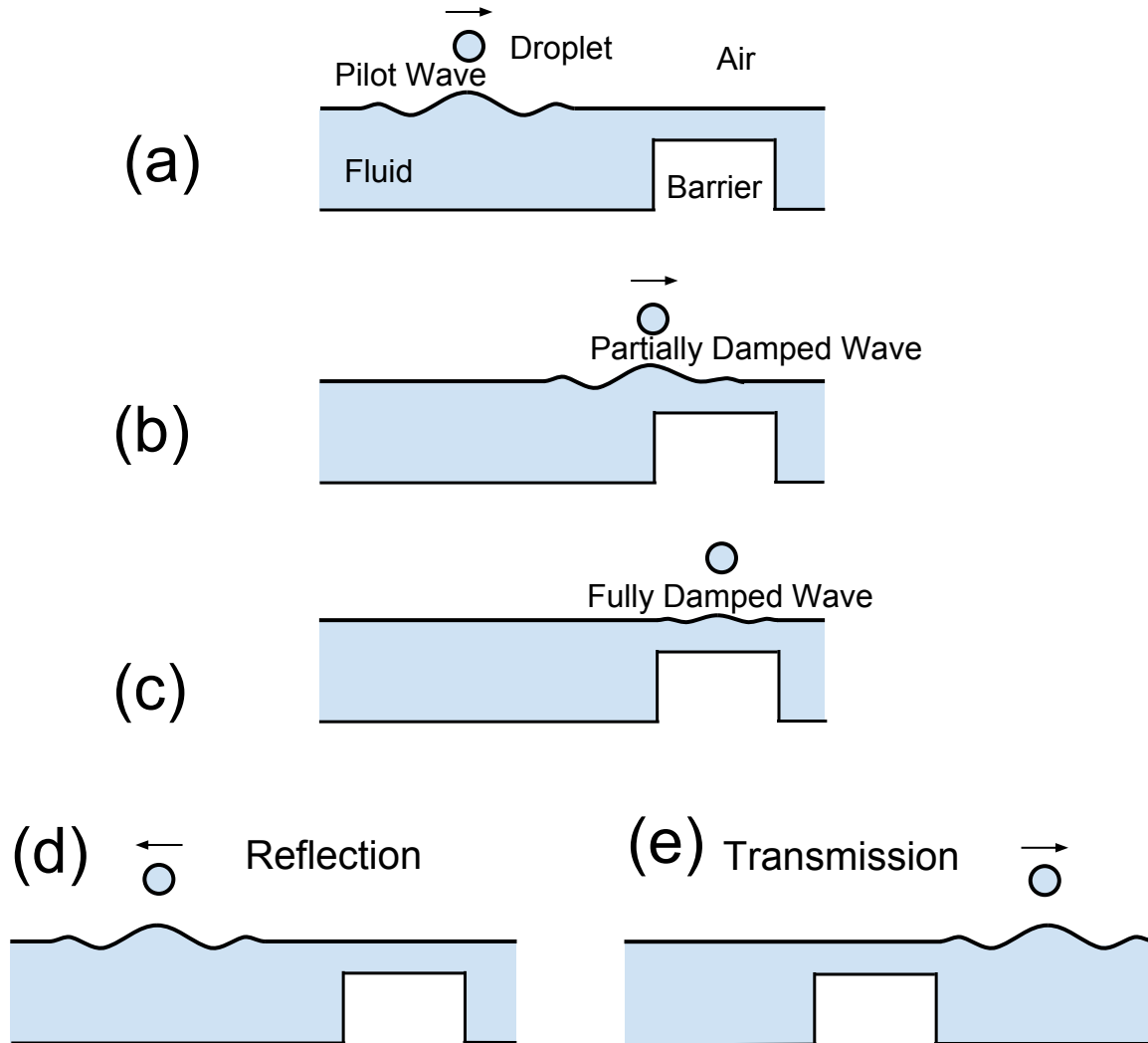
Figure 1.7: A diagram of the droplet-barrier interaction. In (a) the walker moves towards the barrier. As it gets closer (b), the guiding wave is damped. In (c) the guiding wave is fully damped such that the droplet is no longer a walker but a bouncer. Guided by the waves the droplet generated as a walker, the bouncer will either be reflected back from where it came (d), or carry on as shown in (e).
