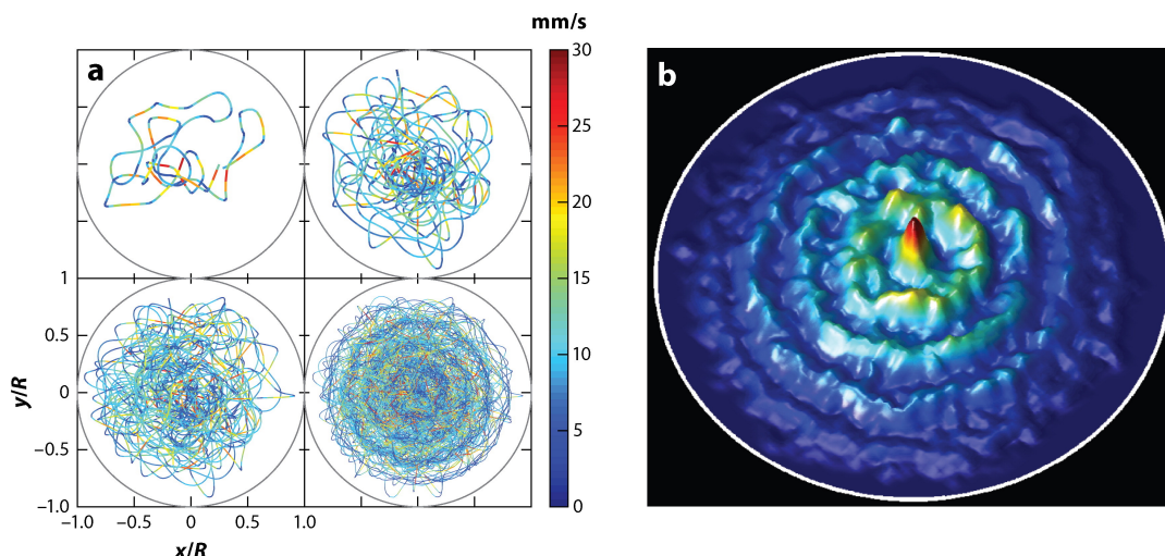
Figure 1.6: The figures show the motion of a single chaotic walker in a confined circular geometry. In (a) the path of the moving droplet is traced, where color indicates the velocity of the droplet. In (b) a histogram shows the droplet’s position within the circular corral over a span of time. A clear pattern emerges: the droplet appears to be contained within a statistical wave of wavelength \lambda_F . Adapted from J. W. M. Bush, Annu. Rev. Fluid Mech. 47 , 275 (2015).
