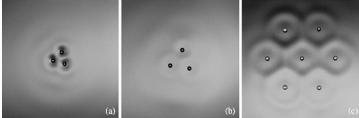
Figure 1.4: In (a), the trio of droplets organize themselves into a triangular lattice separated by distance d_0^{bd} . The forcing acceleration has been increased in (b), and the droplets are more spread out with a larger d_0^{bd} value. Bound states can include a large number of bouncing droplets, as demonstrated by the 7 bouncing droplets shown in (c). Figure from S. Protiere et al., J. Phys.: Condens. Matter 17 , S3532 (2005).
