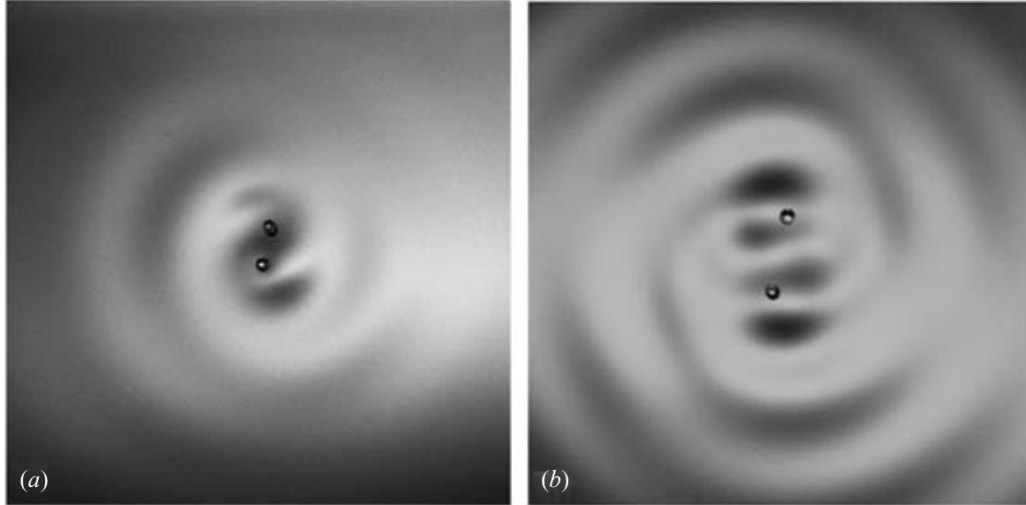
Figure 1.5: The figures show two droplets of equal size orbiting their center of mass. In (a) the droplets bounce out of phase with n = 0.5 and d_n^{orb} = 1.65 mm whereas in (b) the droplets bounce in phase with n = 1 and d_n^{orb} = 3.7 mm. Figure adapted from S. Protiere et al., J. Fluid Mech. 554 , 101 (2006).
