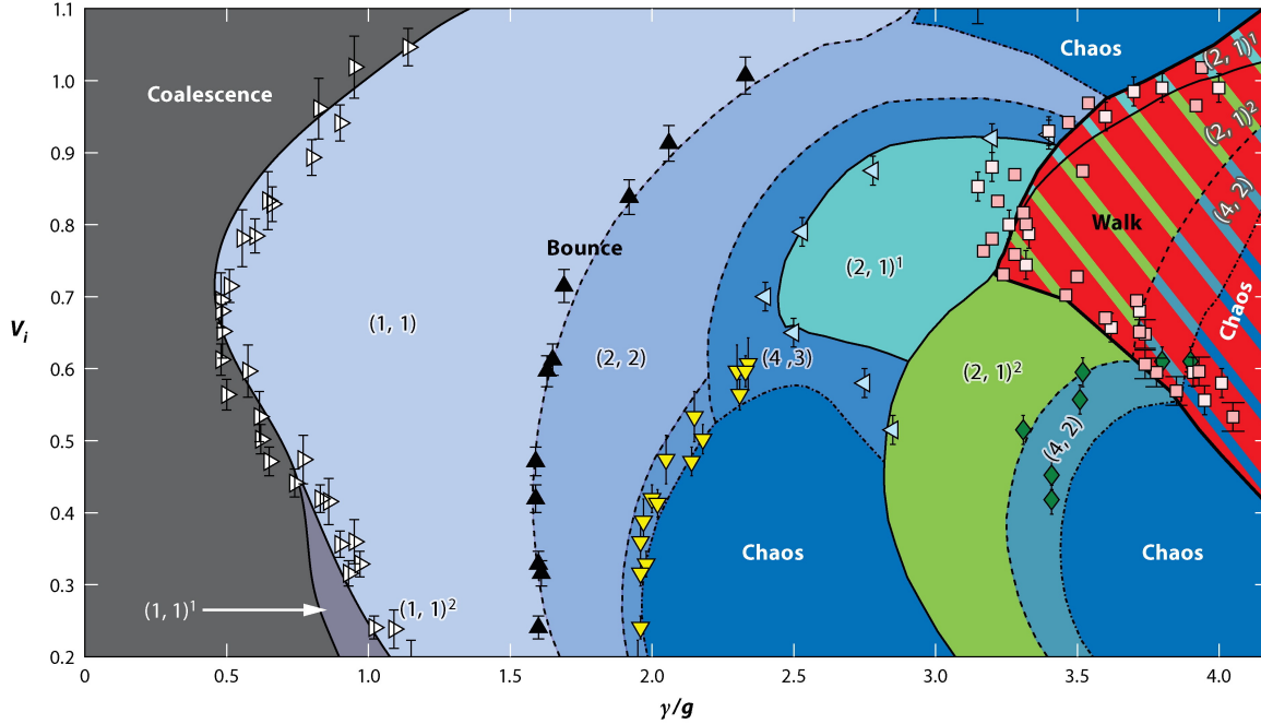
Figure 1.2: The different bouncing regimes for the oil drops of 20 cSt silicone oil at f = \omega/2\pi = 80 Hz, characterized by the non-dimensional forcing amplitude \gamma/g and the vibration number V_i . The solid colors represent the modes predicted by a theoretical model [14], and the various points represent experimentally measured limits. The parameters (m, n)^i describe a droplet that bounces n times in m forcing periods, where i distinguishes modes with different mechanical energy. The Faraday threshold is \gamma_F = 4.2 . Adapted from J. W. M. Bush, Annu. Rev. Fluid Mech. 47 , 273 (2015).
