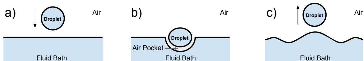
Figure 1: A depiction of a droplet bouncing on a bath of the same fluid. (a) A droplet falls onto a fluid bath. (b) A film of air gets trapped underneath the droplet. (c) The droplet bounces back up off of the cushion of air leaving behind waves that propagate radially.
