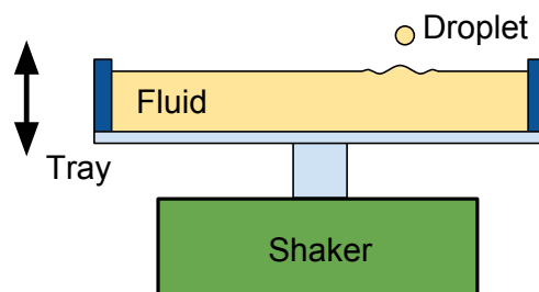
Figure 1.1: A droplet bounces on a vertically vibrating fluid bath. The tray vibrates with an amplitude A_0 at frequency f .
