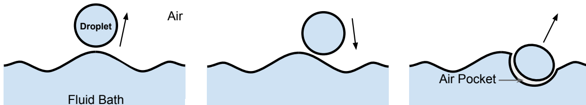
Figure 3: A depiction of a droplet walking across a bath of the same fluid.
