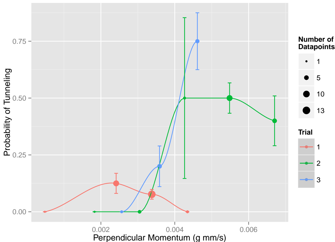
Figure 3.6: Collisions of similar perpendicular momentum were grouped into bins. The overall fraction of transmissions was computed for each bin, and plotted. Colors distinguish between trials, and sizes indicate the number of data points in each bin. Error bars indicate the associated standard error. The droplets were grouped by perpendicular velocities of width 2 mm/s per bin, and then these velocity values were multiplied by m .
