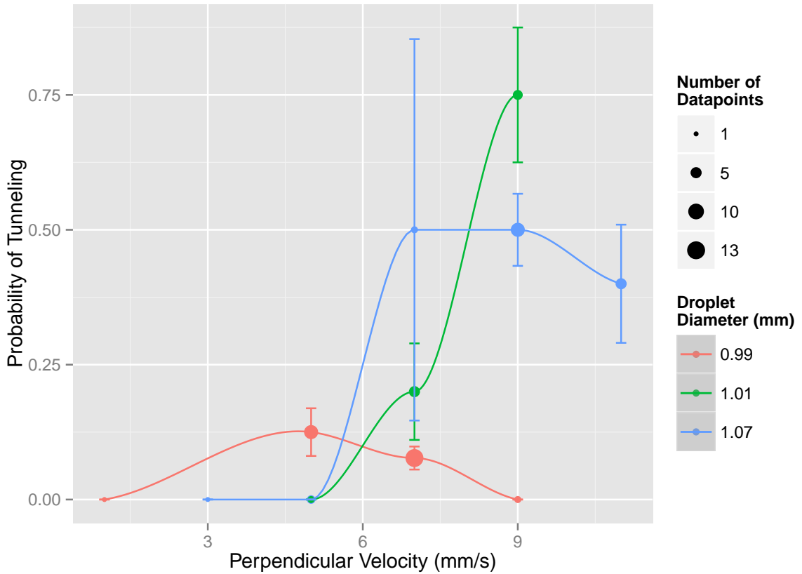
Figure 3.5: Collisions with similar perpendicular velocities were grouped into bins of width 2 mm/s per bin. The overall fraction of transmissions was computed for each bin, and plotted. Colors distinguish between droplet diameters, and sizes indicate the number of data points in each bin. Error bars indicate the associated standard error.
