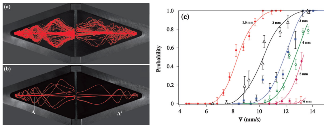
Figure 1.8: In (a) and (b) we see the path of a droplet traced out over many collisions with the barrier within rhombus shaped tray. The plot (c) shows the tunneling probability as a function of walker velocity for different barrier widths. Figures adapted from A. Eddi et al., Phys. Rev. Lett. 102 , 240401 (2009).
