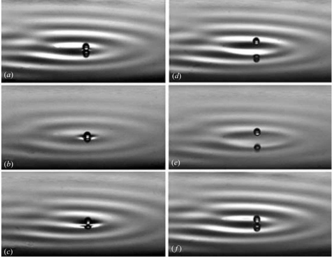
Figure 1.3: The series of pictures (a) - (f) show a walker over two forcing periods. The droplet bounces off of the slope of the localized wave, launching into the air, and then falls again on a new wave slope. This periodic process happens multiple times per second, giving the droplet the appearance of walking across the surface. Figure from S. Protiere et al., J. Fluid Mech. 554 , 93 (2006).
