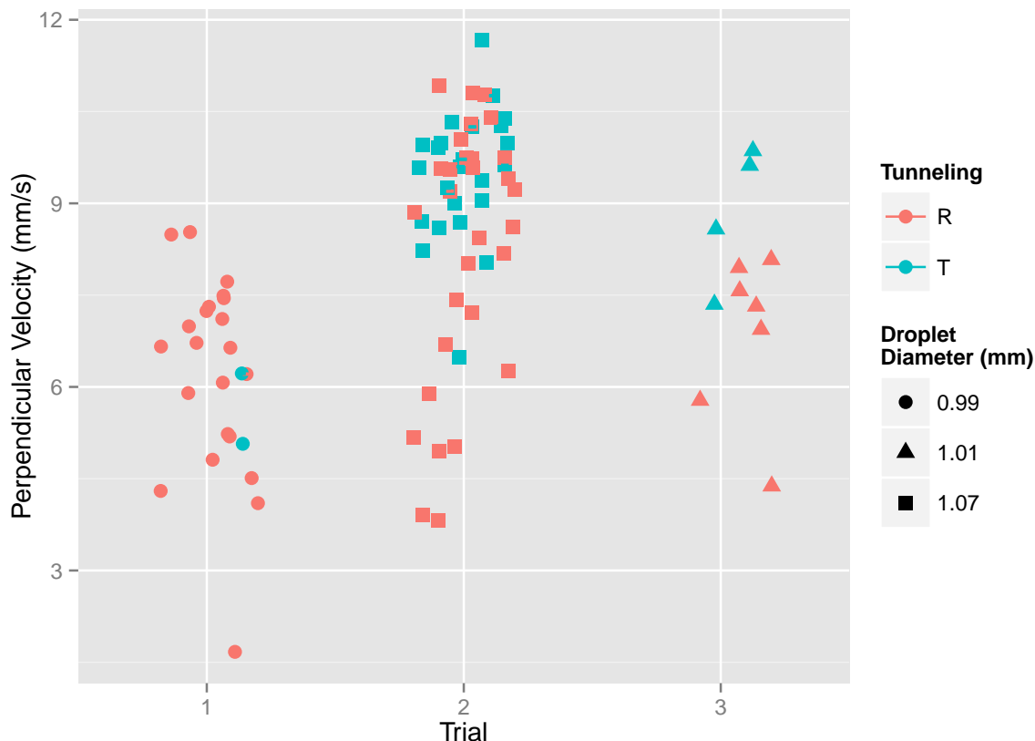
Figure 3.4: The result of each collision for the intermediate oil depth. The color represents the outcome of the collision (either transmission (T) or reflection (R)), and the shape represents the diameter of the droplet. The horizontal spread within each trial was added to aid in visualization.
