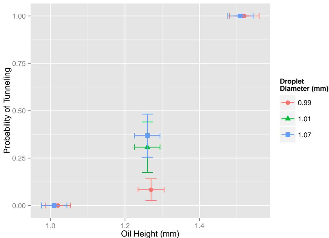
Figure 3.2: The proportion of collisions leading to transmission as a function of h . Each data series corresponds to a single trial for which the droplet diameter was kept constant. The vertical error bars indicate standard error, and the horizontal error bars indicate uncertainty calculated using error propagation.
