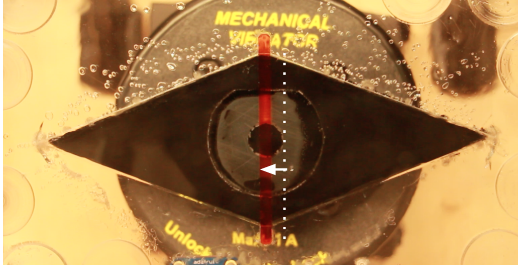
Figure 3.3: The image shows the point at which the measurement of the perpendicular component of velocity was made. This is 5 mm from the middle of the barrier.
