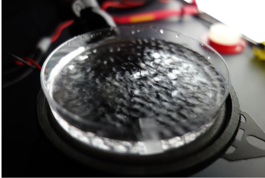
Figure 2: A picture of Faraday waves in a dish of water at 80 Hz.
