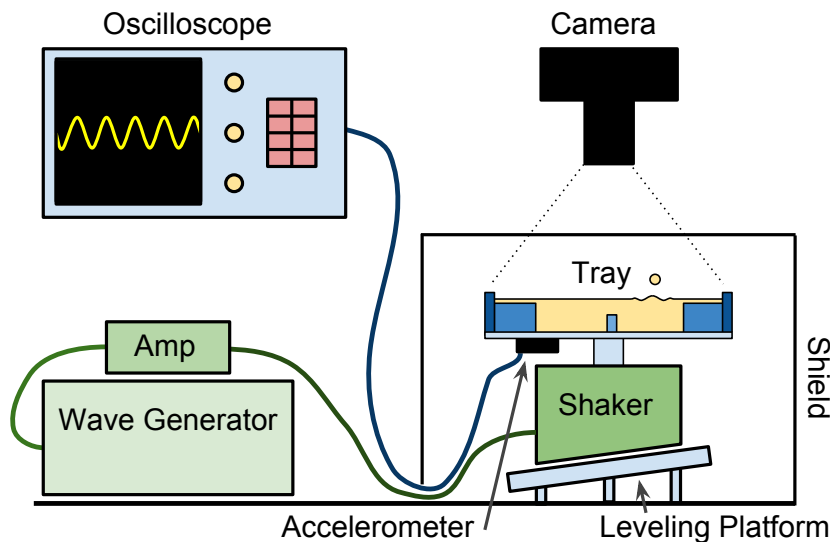
Figure 2.1: The experimental setup. The amplified signal from the wave generator drives the shaker, which shakes the oil-filled tray. The accelerometer generates a signal, which is read by the oscilloscope. The shield blocks disturbances to the experiment, while allowing the camera to document the trials.
