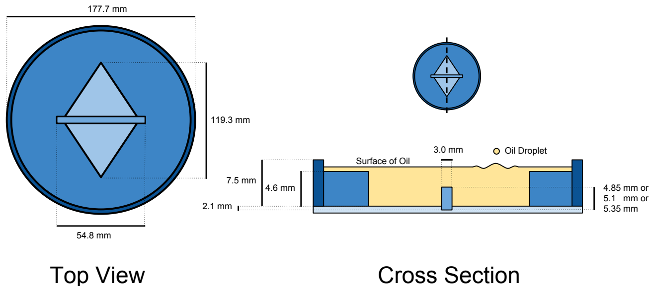
Figure 2.2: The specifications of the tray design. The top view (left) highlights the main elements in the tray. The cross section (right) illustrates the topography of the tray. The depth of the fluid layer is represented by the shading; darker shading is shallower.
